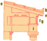
Structure of Doric entablature
